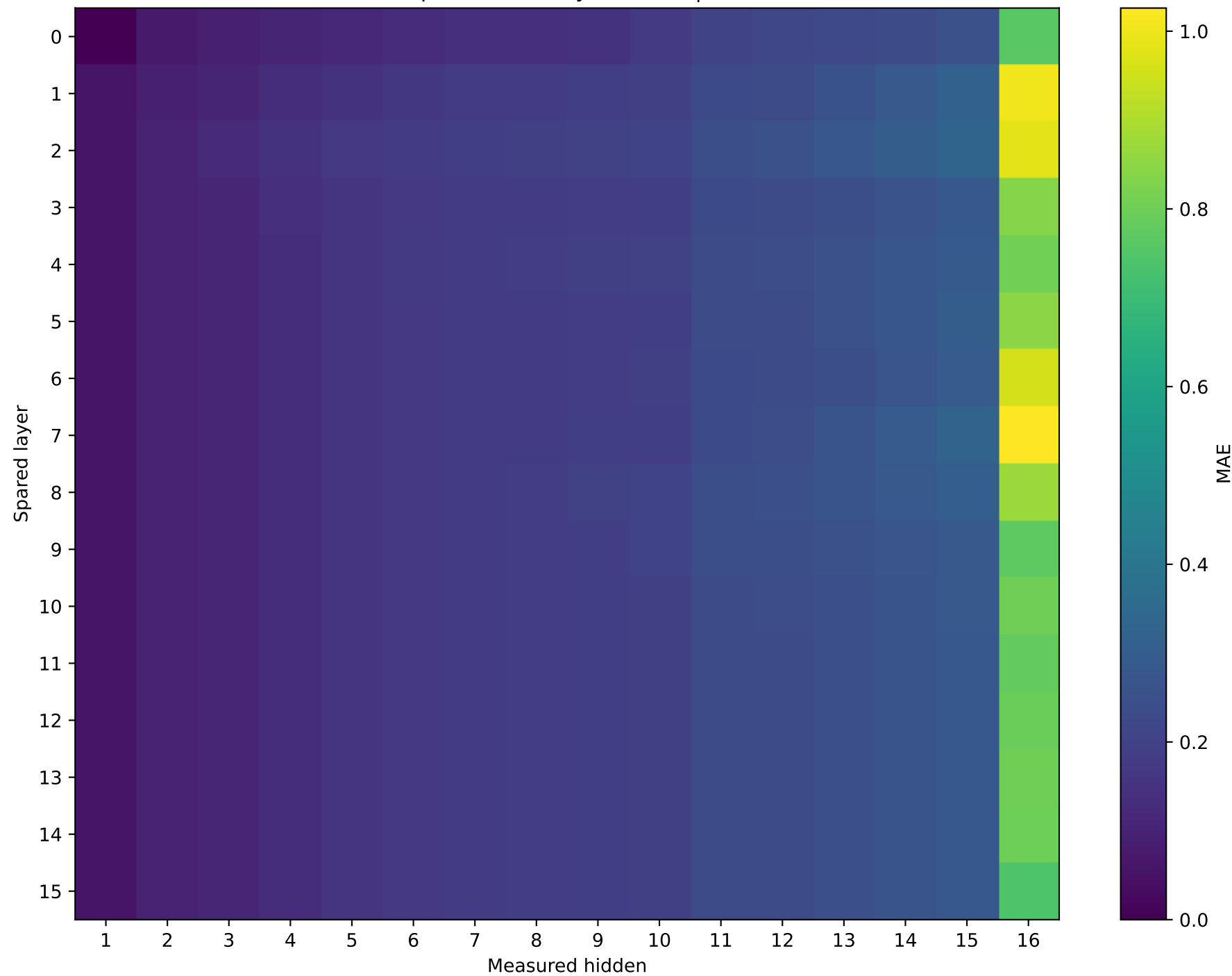
OLMo-1B-hf | Prompt 1 Unquantized vs hybrid MAE | int4
