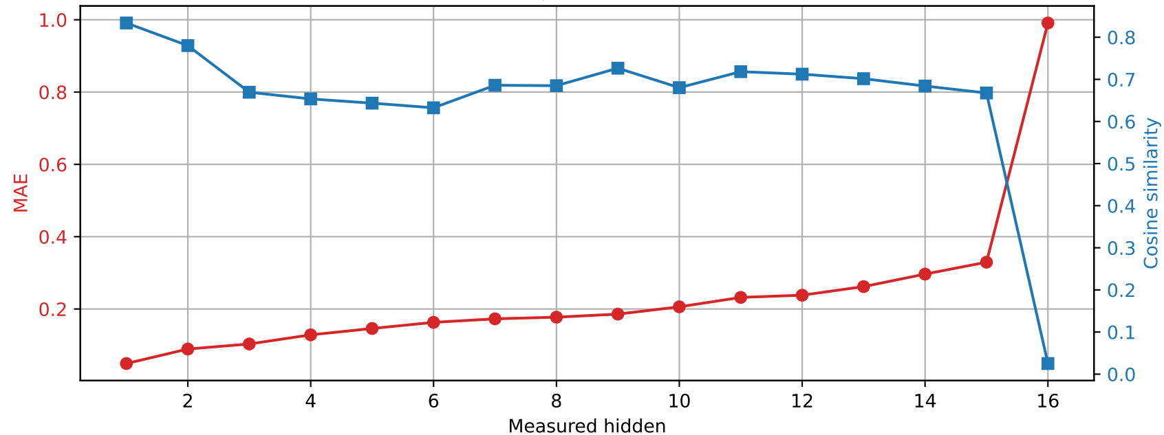
OLMo-1B-hf | Prompt 2 Spared layer 1 | Unquantized vs hybrid
