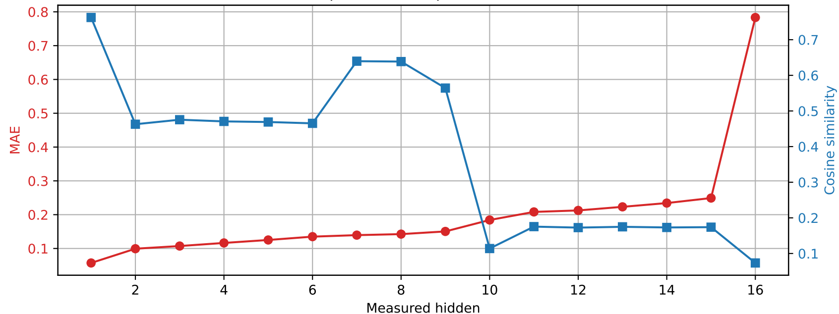
OLMo-1B-hf | Prompt 3 Unquantized vs quantized int4
