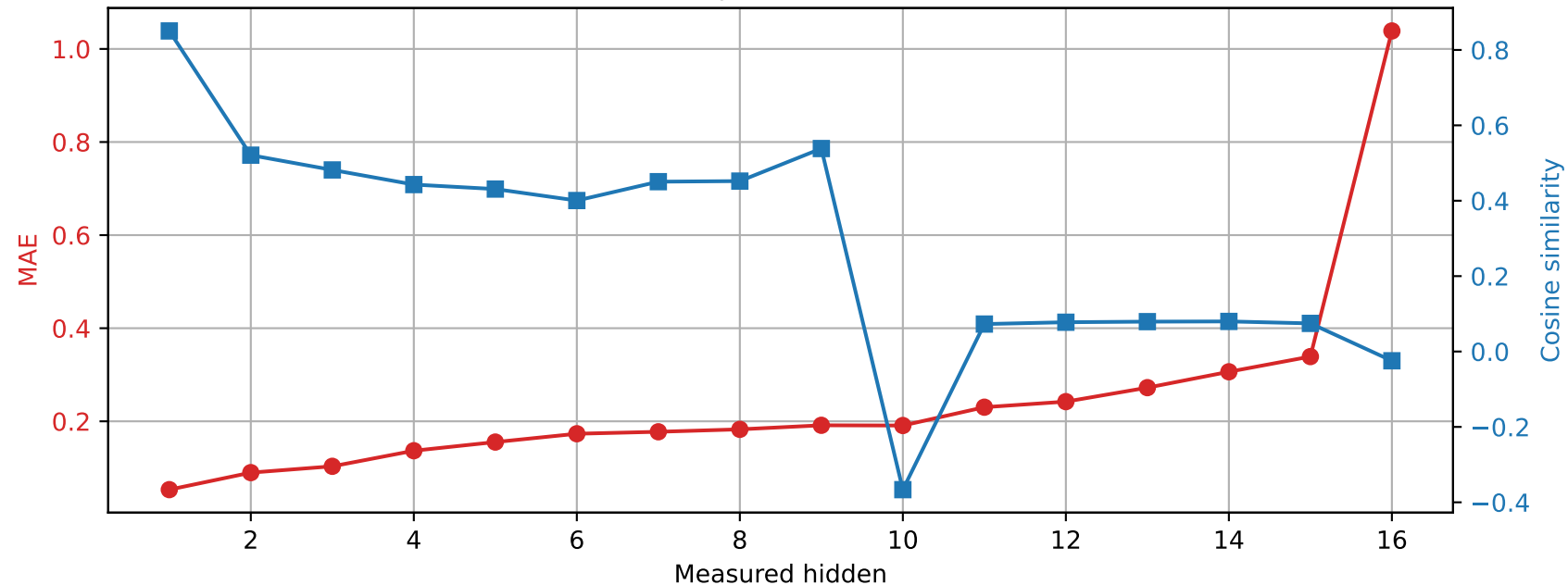
OLMo-1B-hf | Prompt 4 Spared layer 6 | Unquantized vs hybrid
