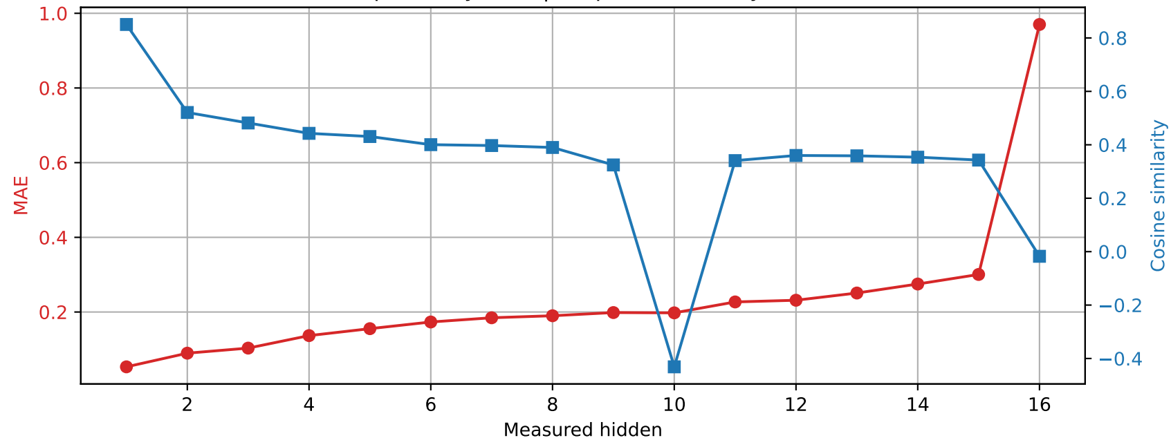
OLMo-1B-hf | Prompt 4 Spared layer 10 | Unquantized vs hybrid
