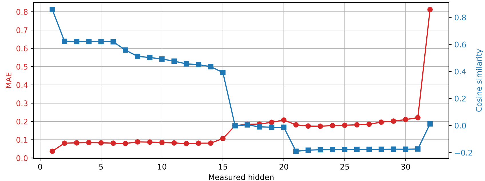
OLMo-7B-hf | Prompt 0 Spared layer 10 | Unquantized vs hybrid
