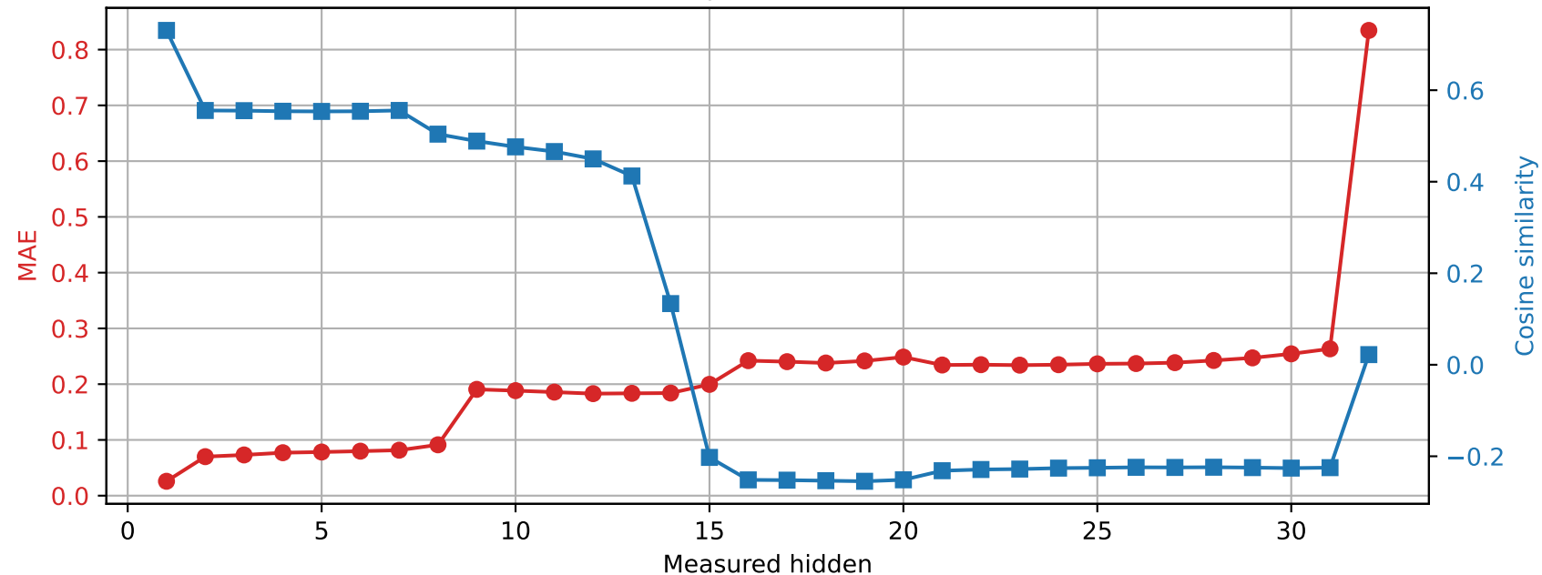
OLMo-7B-hf | Prompt 1 Spared layer 8 | Unquantized vs hybrid
