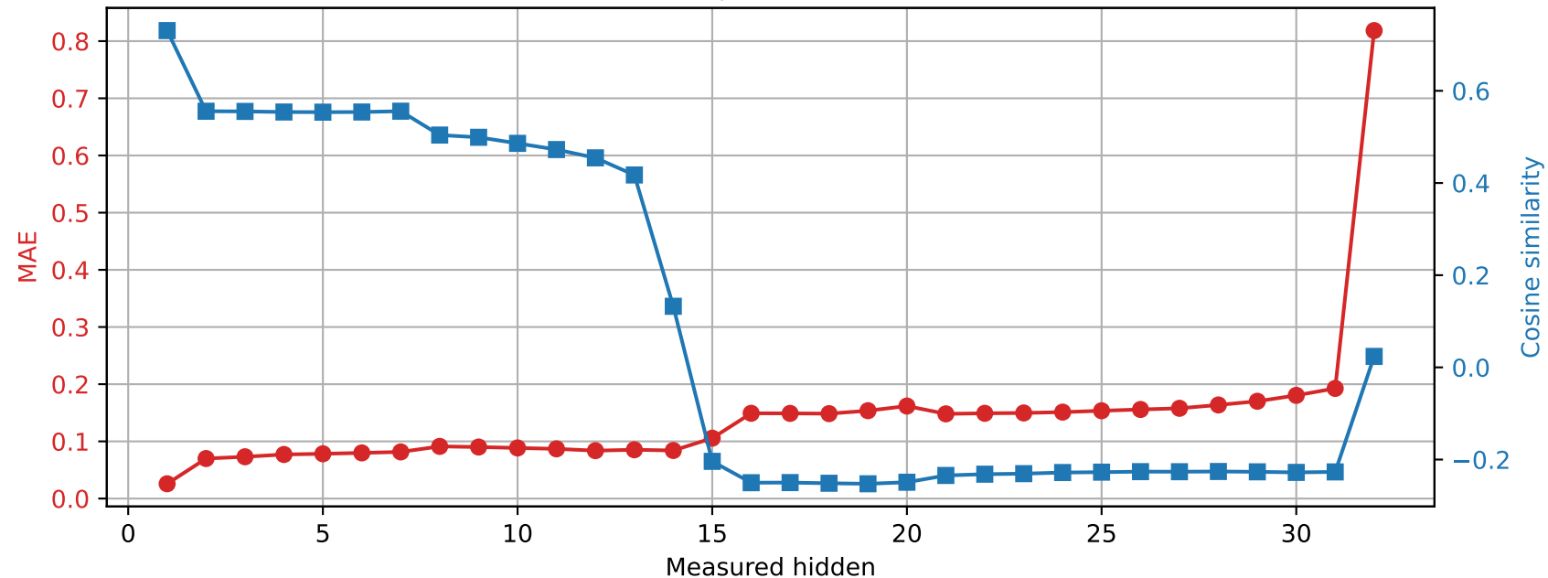
OLMo-7B-hf | Prompt 1 Spared layer 14 | Unquantized vs hybrid
