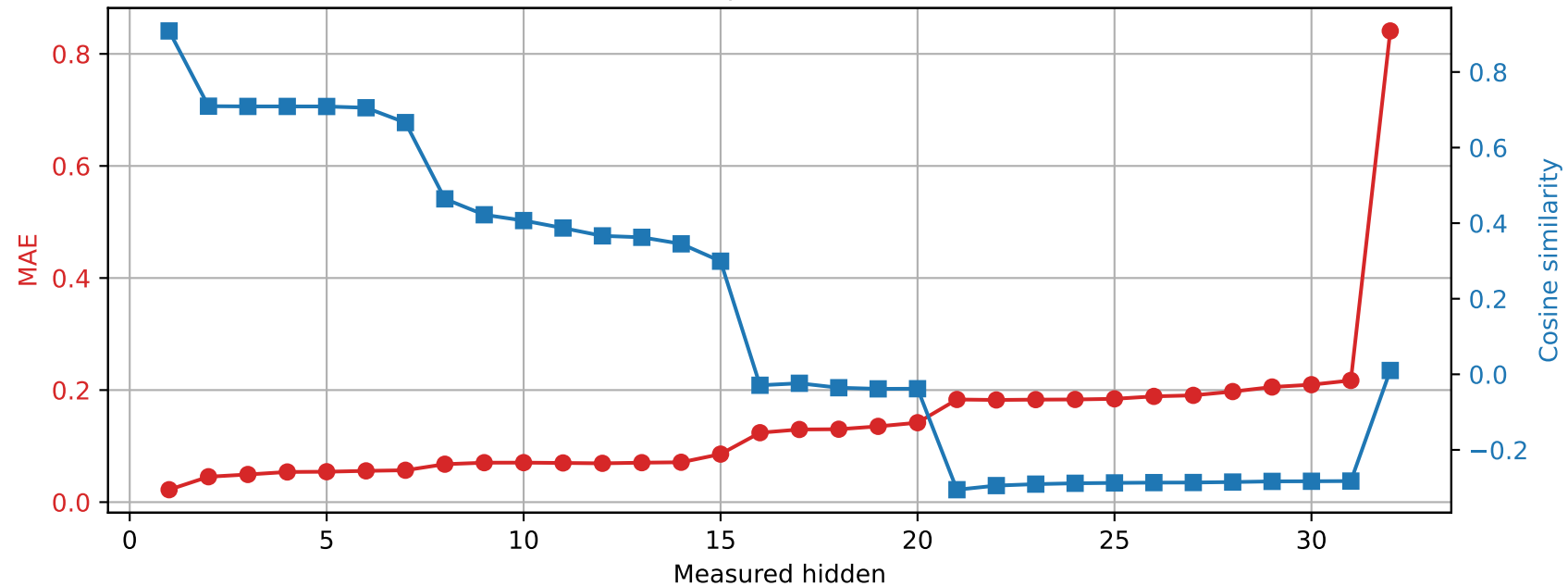
OLMo-7B-hf | Prompt 2 Spared layer 20 | Unquantized vs hybrid
