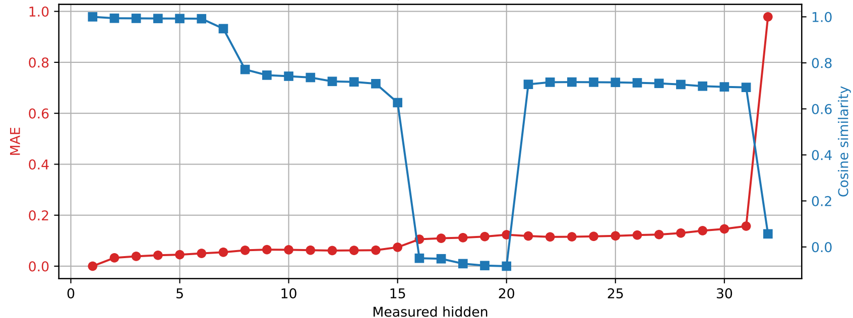
OLMo-7B-hf | Prompt 3 Spared layer 0 | Unquantized vs hybrid
