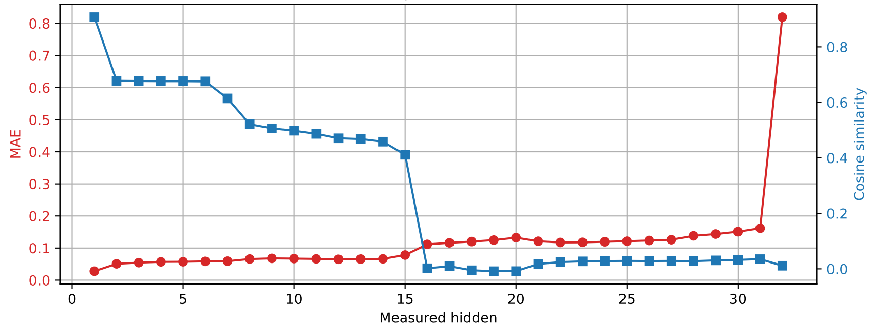
OLMo-7B-hf | Prompt 3 Spared layer 5 | Unquantized vs hybrid
