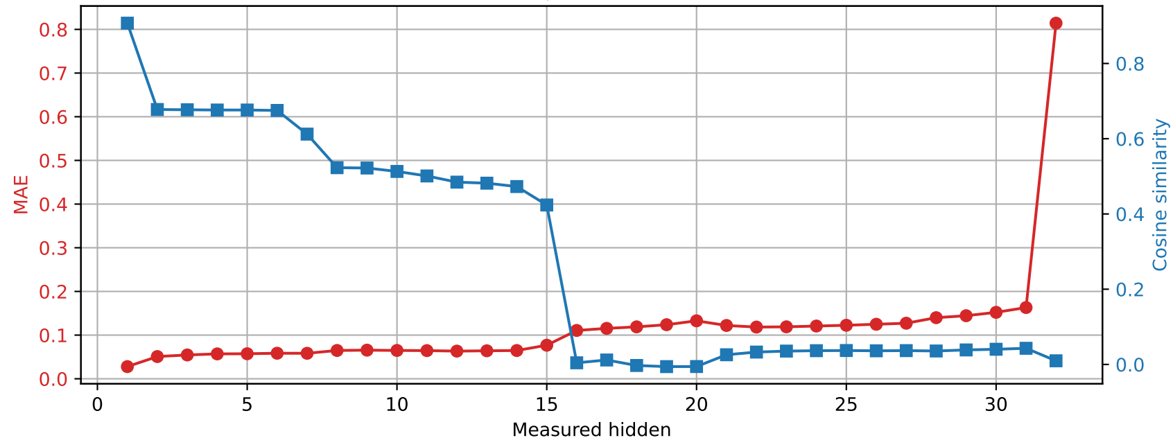
OLMo-7B-hf | Prompt 3 Spared layer 6 | Unquantized vs hybrid
