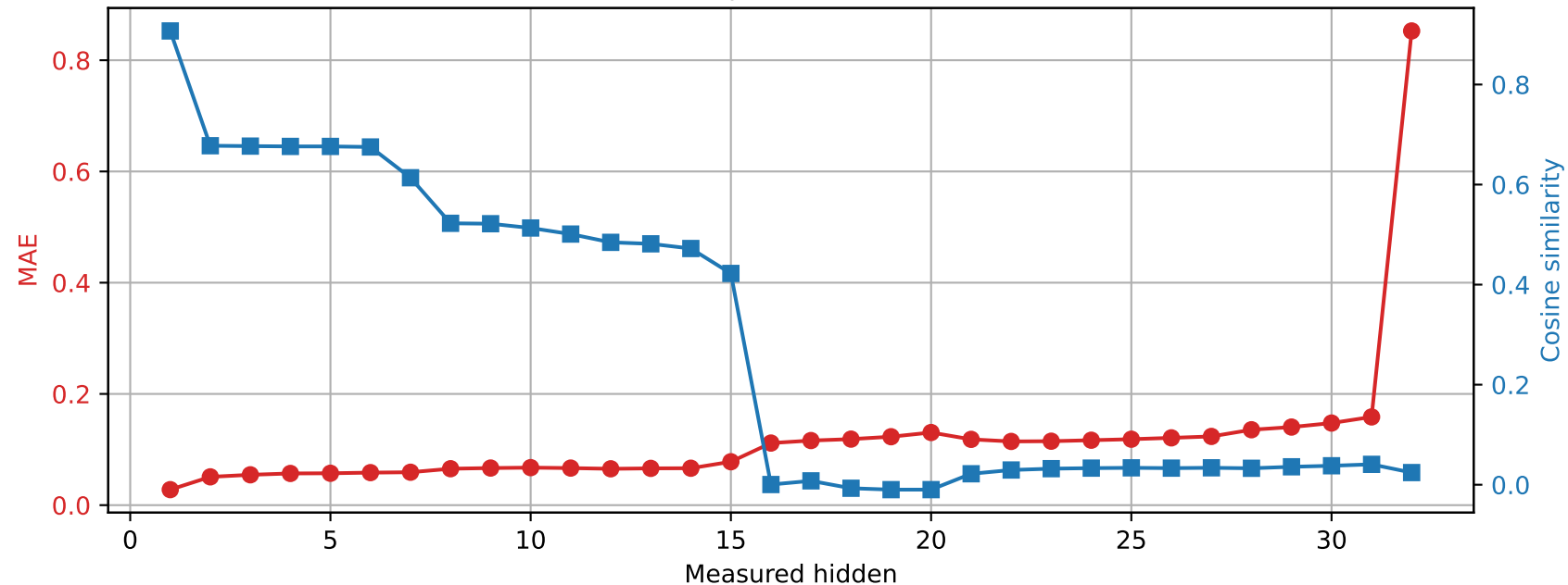
OLMo-7B-hf | Prompt 3 Spared layer 9 | Unquantized vs hybrid
