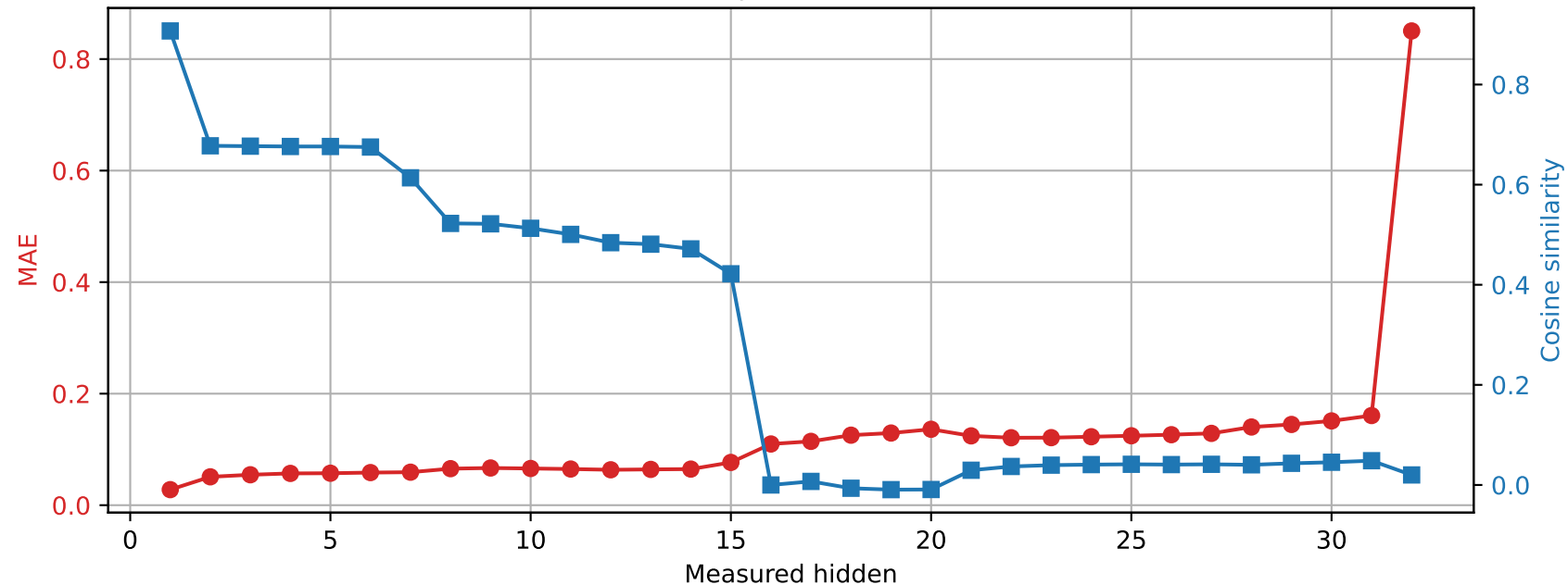
OLMo-7B-hf | Prompt 3 Spared layer 17 | Unquantized vs hybrid
