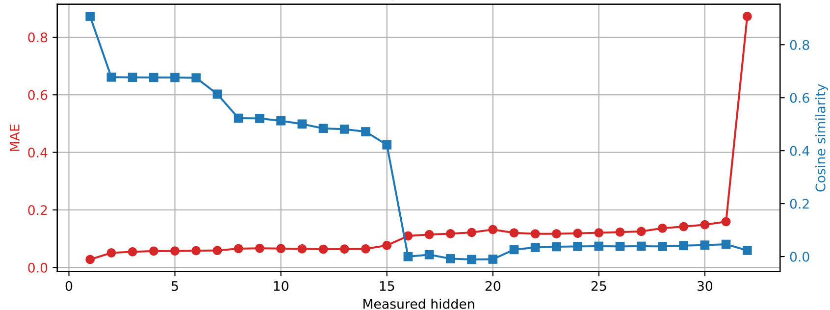
OLMo-7B-hf | Prompt 3 Spared layer 19 | Unquantized vs hybrid
