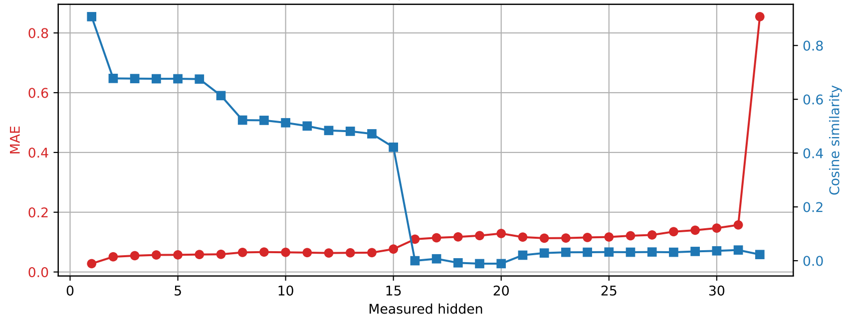
OLMo-7B-hf | Prompt 3 Spared layer 23 | Unquantized vs hybrid
