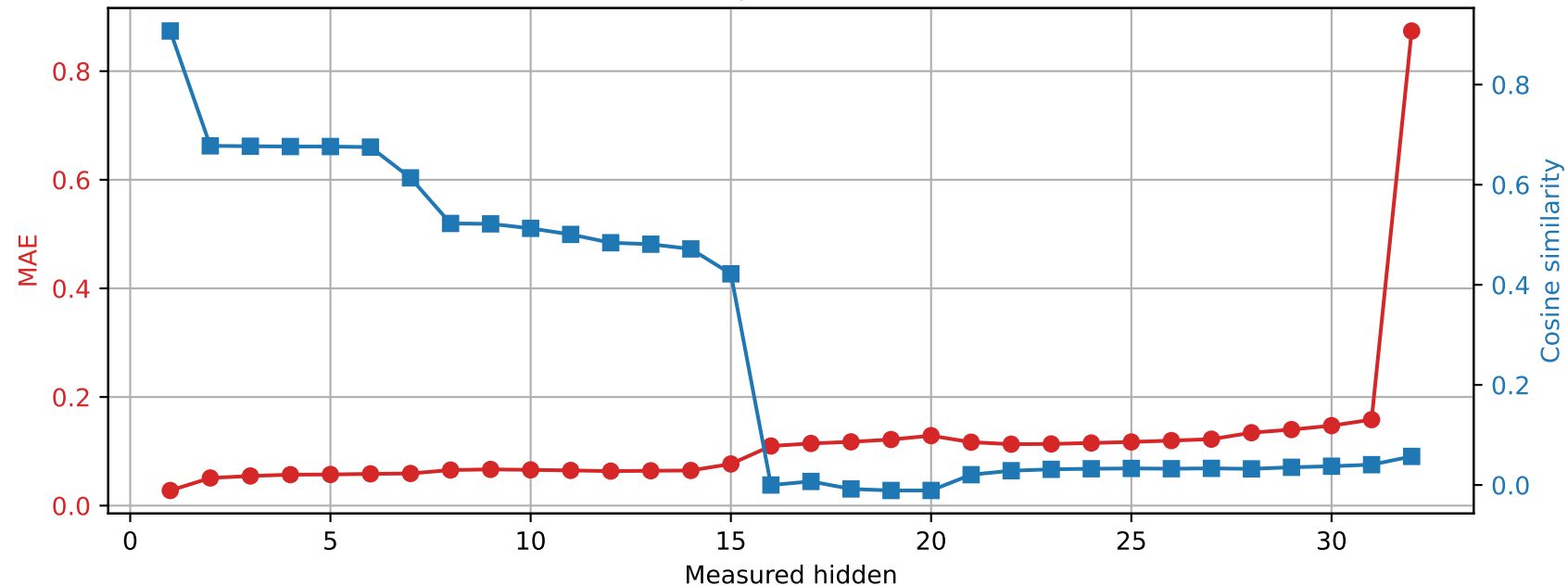
OLMo-7B-hf | Prompt 3 Spared layer 31 | Unquantized vs hybrid
