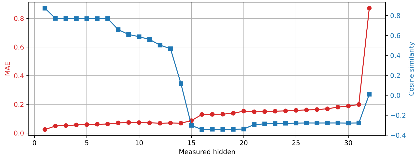
OLMo-7B-hf | Prompt 4 Spared layer 19 | Unquantized vs hybrid
