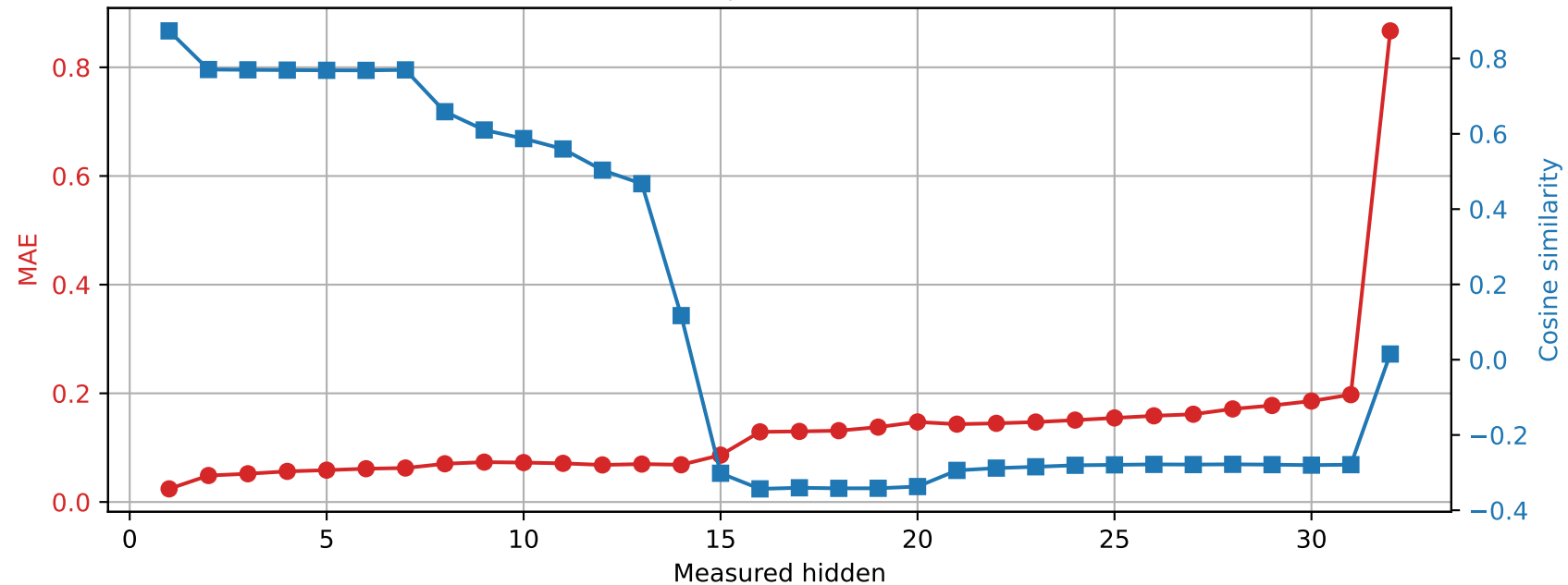
OLMo-7B-hf | Prompt 4 Spared layer 23 | Unquantized vs hybrid
