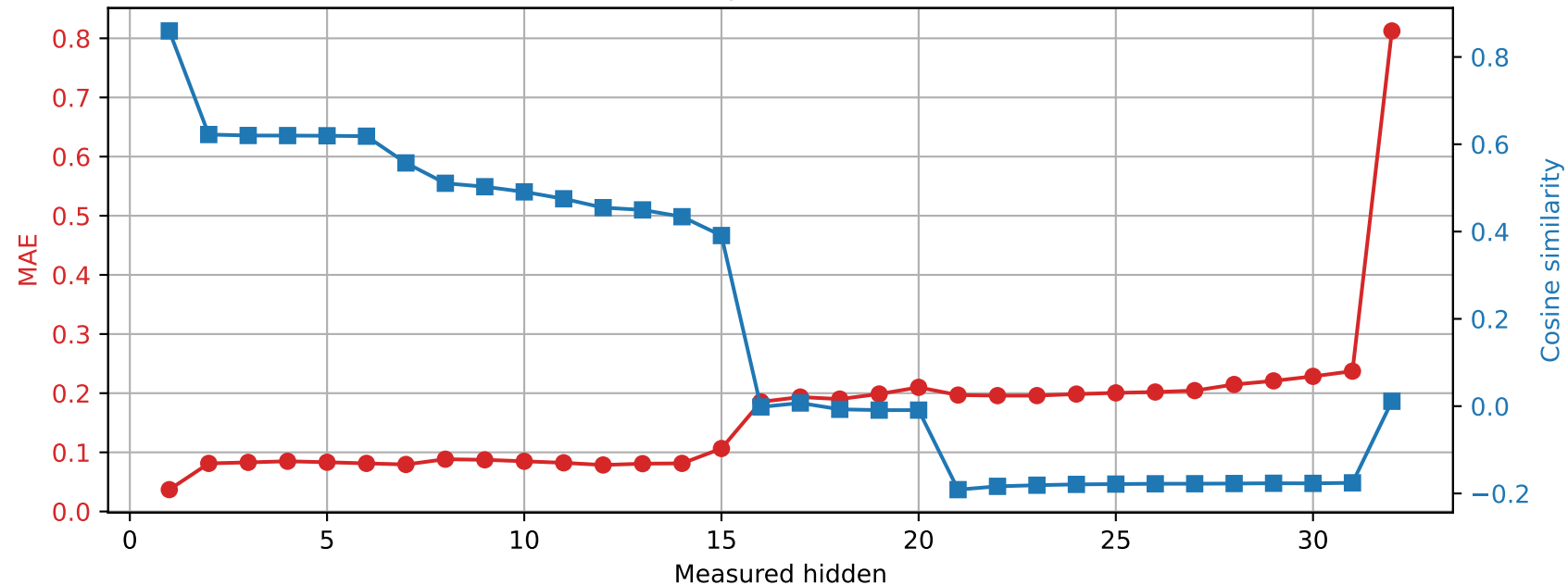
OLMo-7B-hf | Prompt 0 Spared layer 15 | Unquantized vs hybrid
