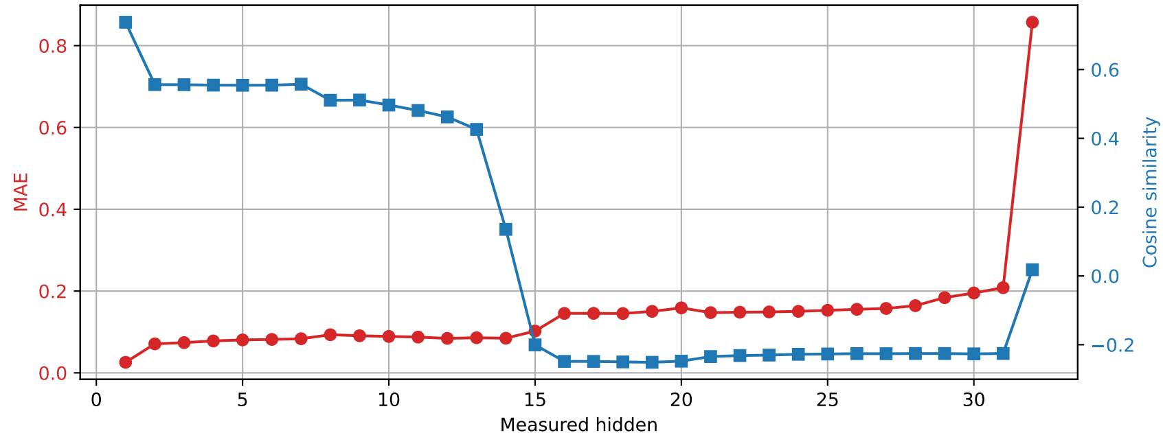
OLMo-7B-hf | Prompt 1 Spared layer 4 | Unquantized vs hybrid
