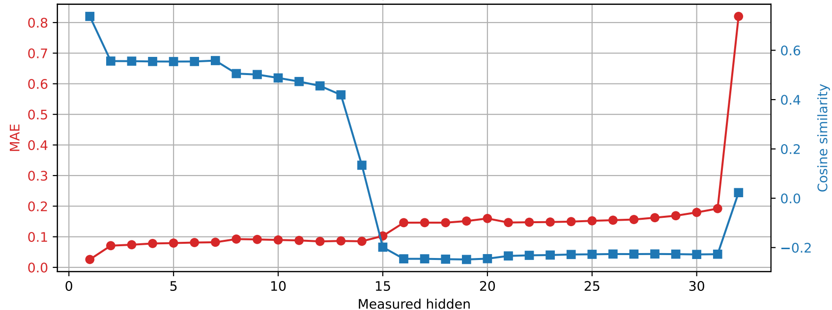
OLMo-7B-hf | Prompt 1 Spared layer 6 | Unquantized vs hybrid
