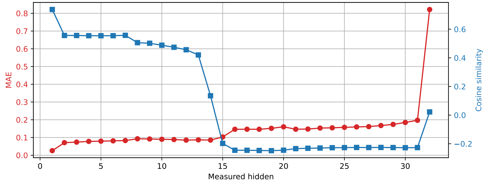
OLMo-7B-hf | Prompt 1 Spared layer 22 | Unquantized vs hybrid
