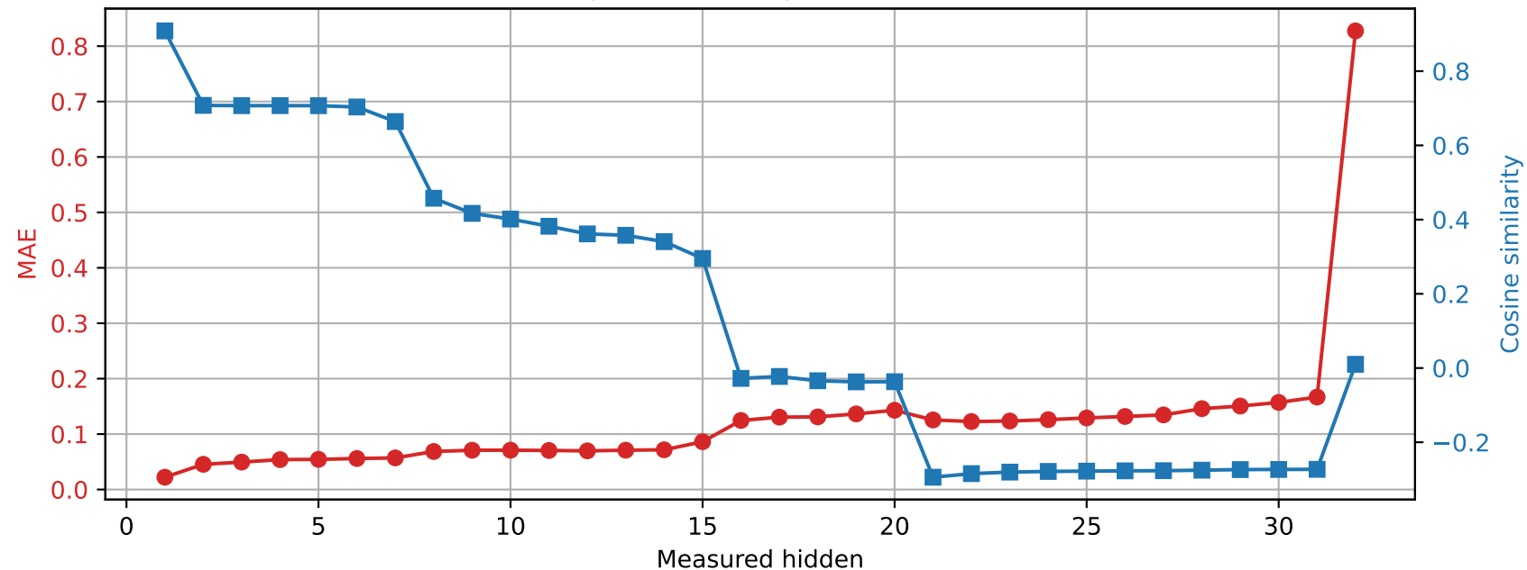
OLMo-7B-hf | Prompt 2 Unquantized vs quantized int4
