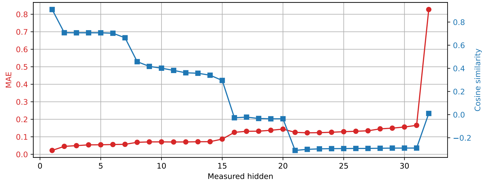
OLMo-7B-hf | Prompt 2 Spared layer 11 | Unquantized vs hybrid
