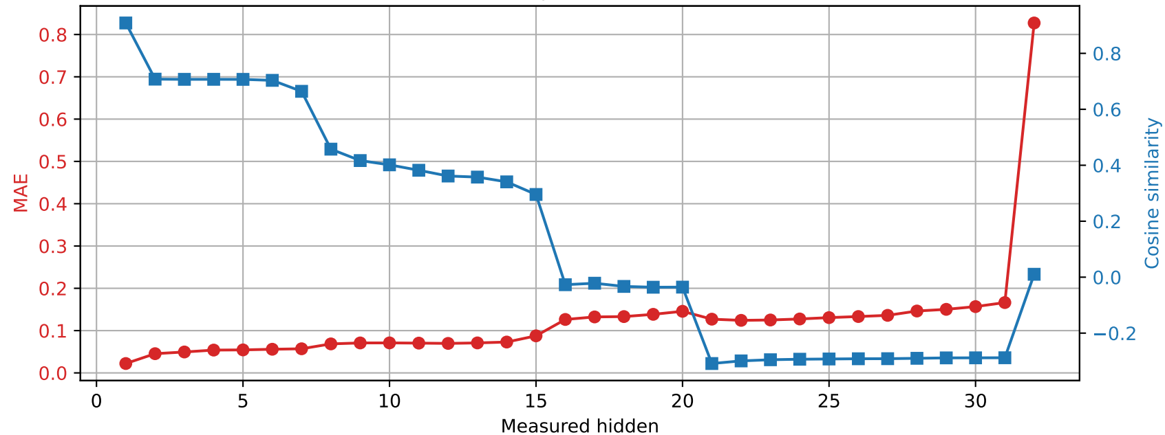
OLMo-7B-hf | Prompt 2 Spared layer 13 | Unquantized vs hybrid
