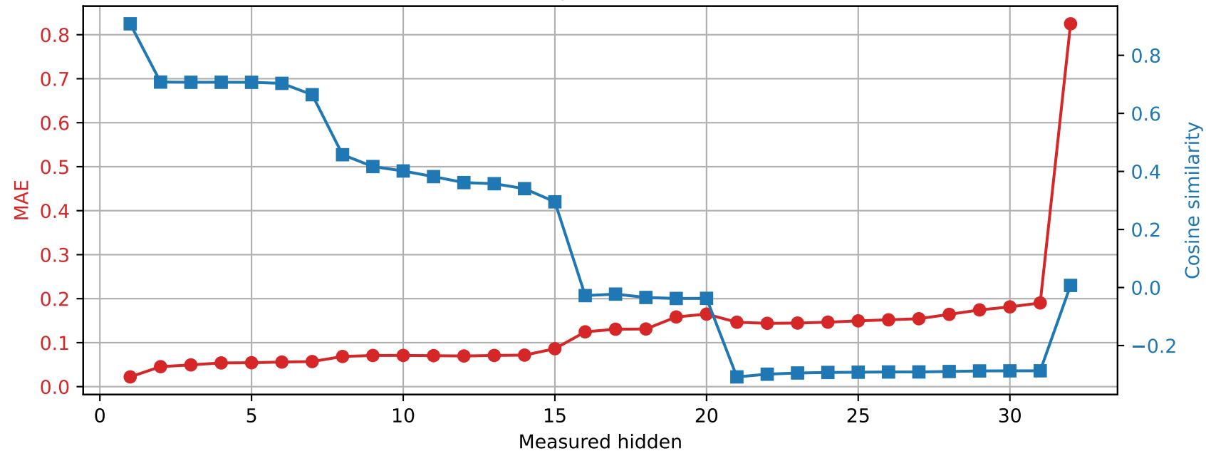
OLMo-7B-hf | Prompt 2 Spared layer 18 | Unquantized vs hybrid
