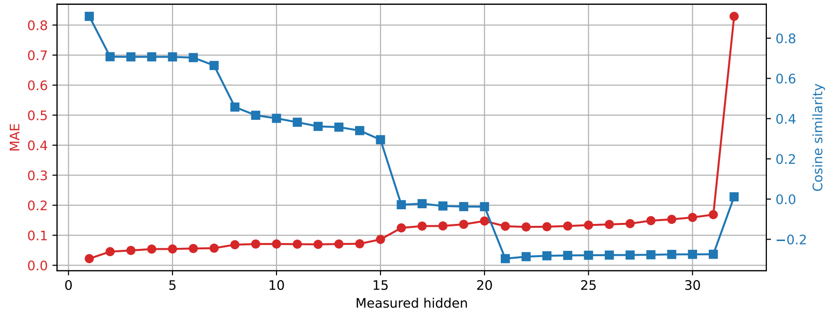
OLMo-7B-hf | Prompt 2 Spared layer 19 | Unquantized vs hybrid
