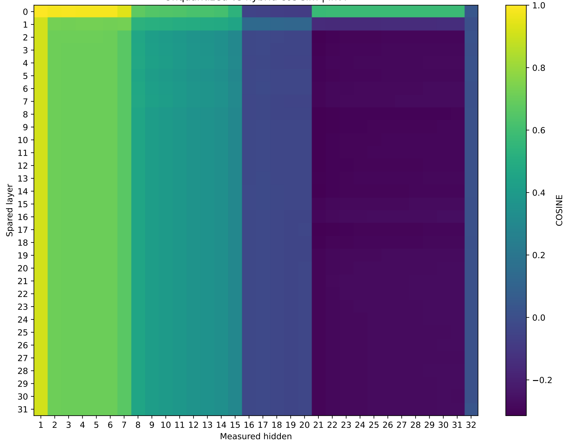
OLMo-7B-hf | Prompt 2 Unquantized vs hybrid cos sim | int4
