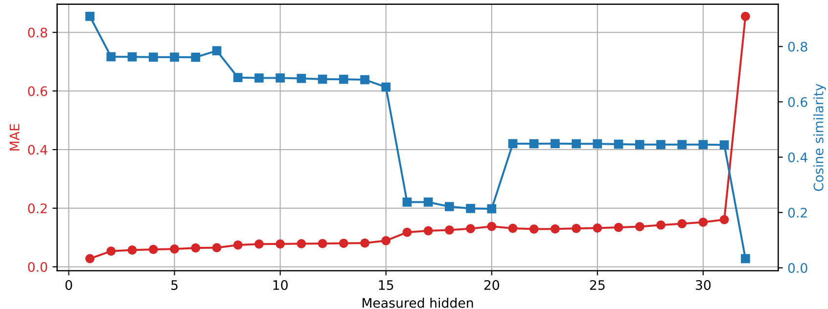
OLMo-7B-hf | Prompt 3 Spared layer 1 | Unquantized vs hybrid
