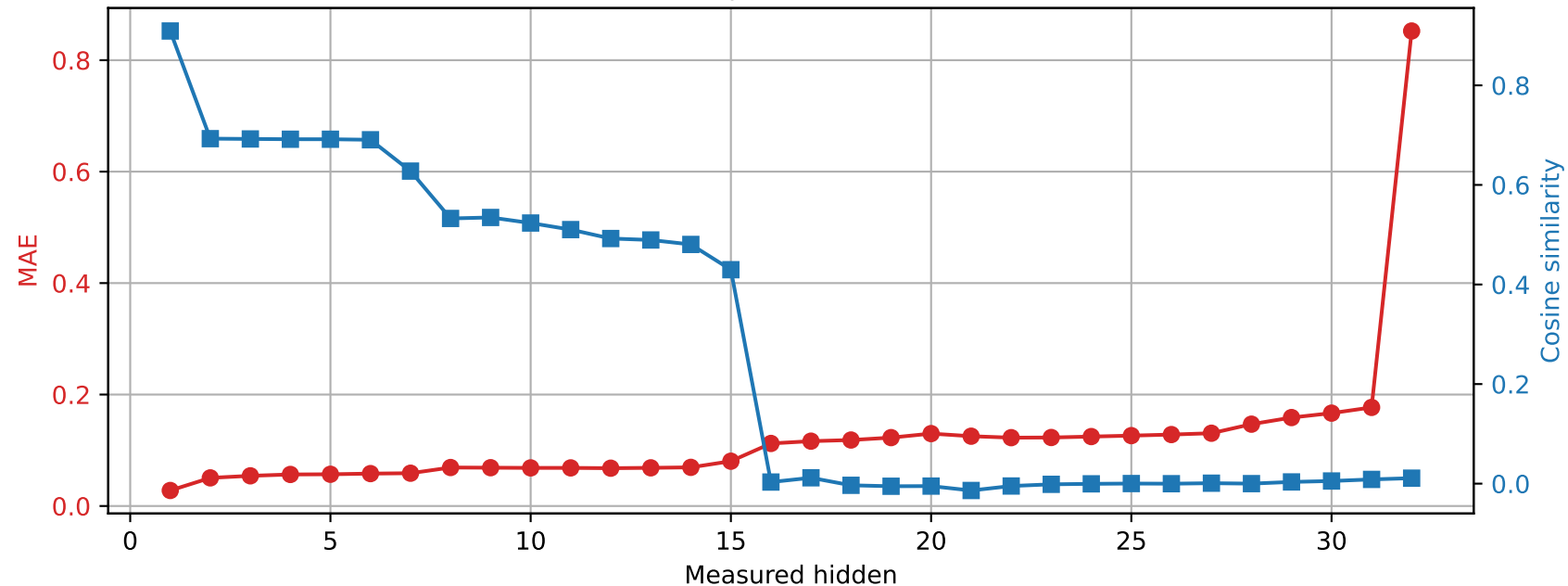
OLMo-7B-hf | Prompt 3 Spared layer 7 | Unquantized vs hybrid
