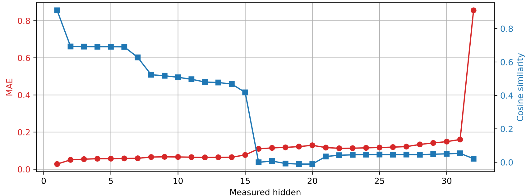
OLMo-7B-hf | Prompt 3 Spared layer 25 | Unquantized vs hybrid
