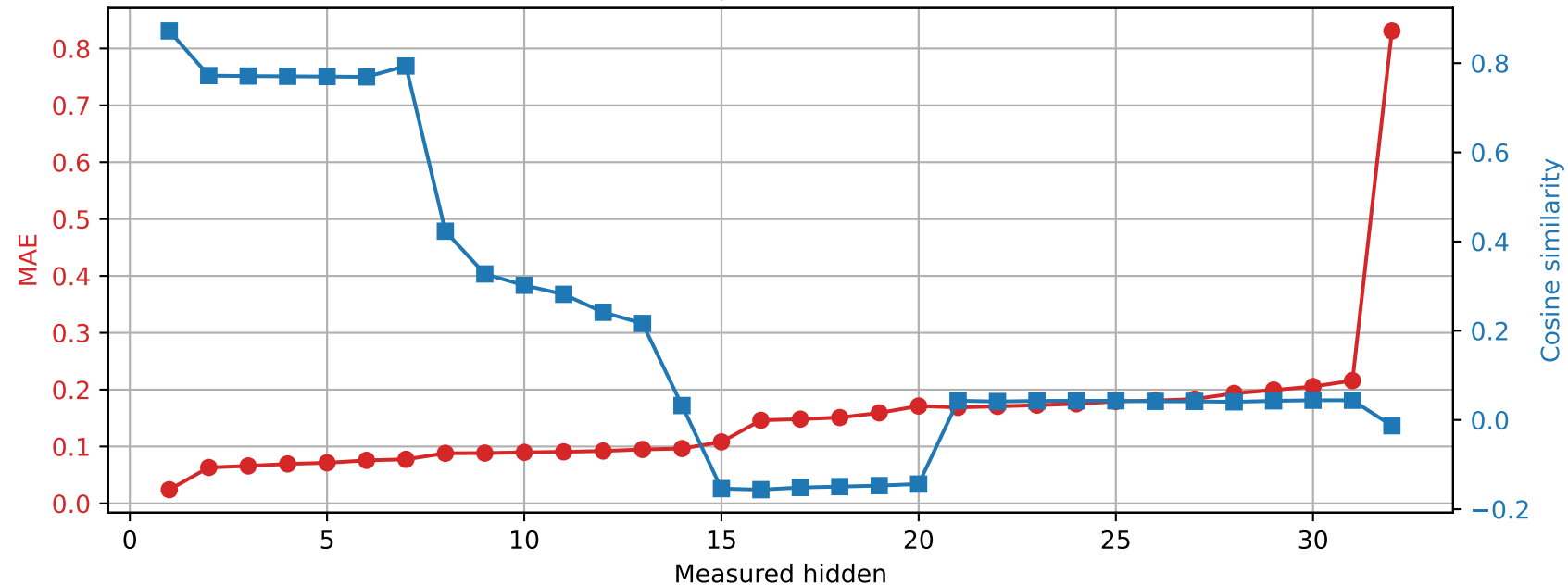
OLMo-7B-hf | Prompt 4 Spared layer 1 | Unquantized vs hybrid
