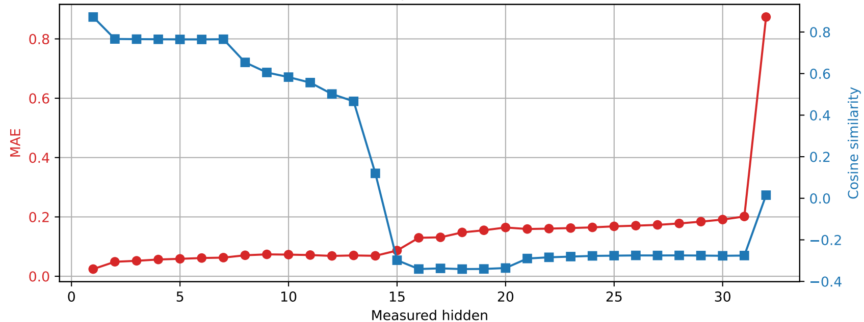
OLMo-7B-hf | Prompt 4 Spared layer 17 | Unquantized vs hybrid
