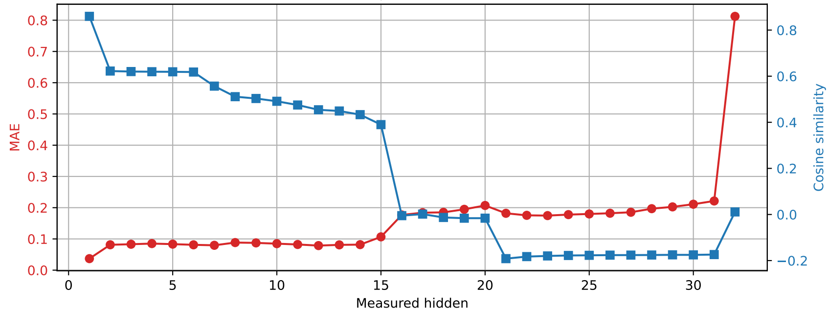
OLMo-7B-hf | Prompt 0 Spared layer 3 | Unquantized vs hybrid
