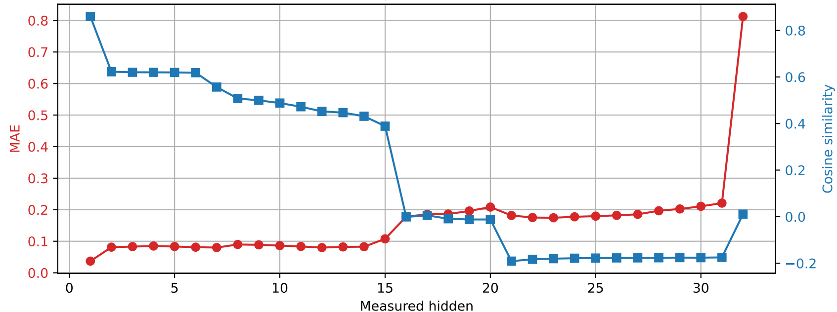
OLMo-7B-hf | Prompt 0 Spared layer 5 | Unquantized vs hybrid
