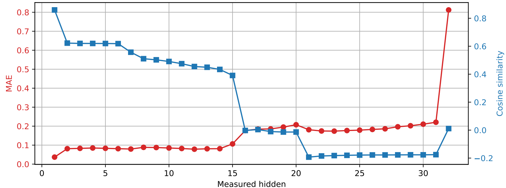
OLMo-7B-hf | Prompt 0 Spared layer 24 | Unquantized vs hybrid
