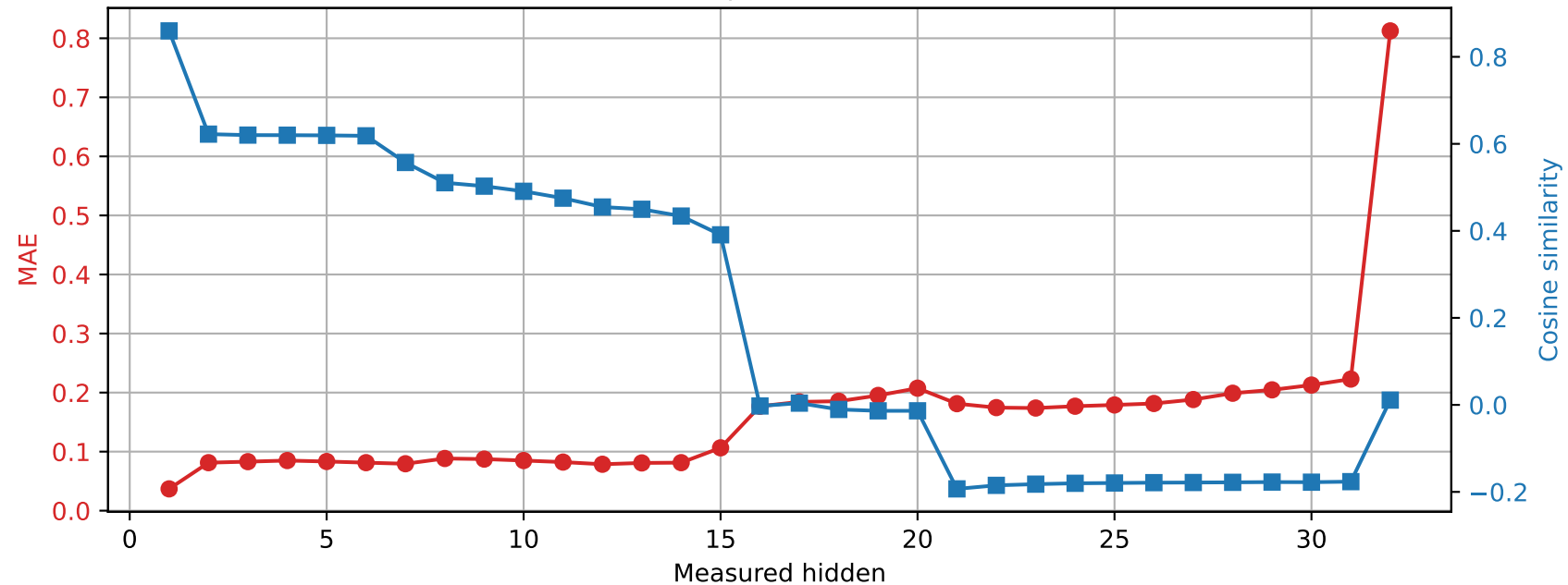
OLMo-7B-hf | Prompt 0 Spared layer 26 | Unquantized vs hybrid
