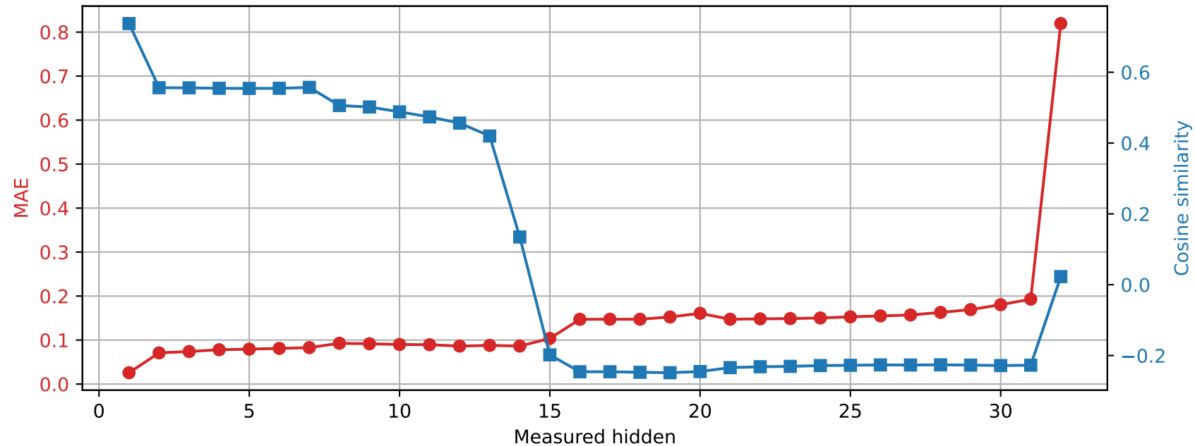
OLMo-7B-hf | Prompt 1 Spared layer 10 | Unquantized vs hybrid
