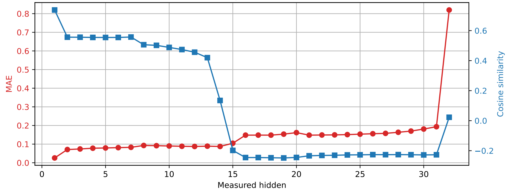
OLMo-7B-hf | Prompt 1 Spared layer 11 | Unquantized vs hybrid
