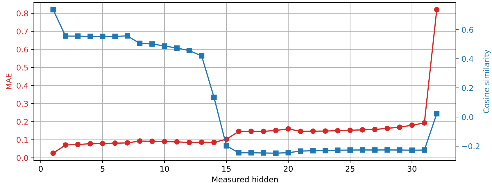
OLMo-7B-hf | Prompt 1 Spared layer 23 | Unquantized vs hybrid
