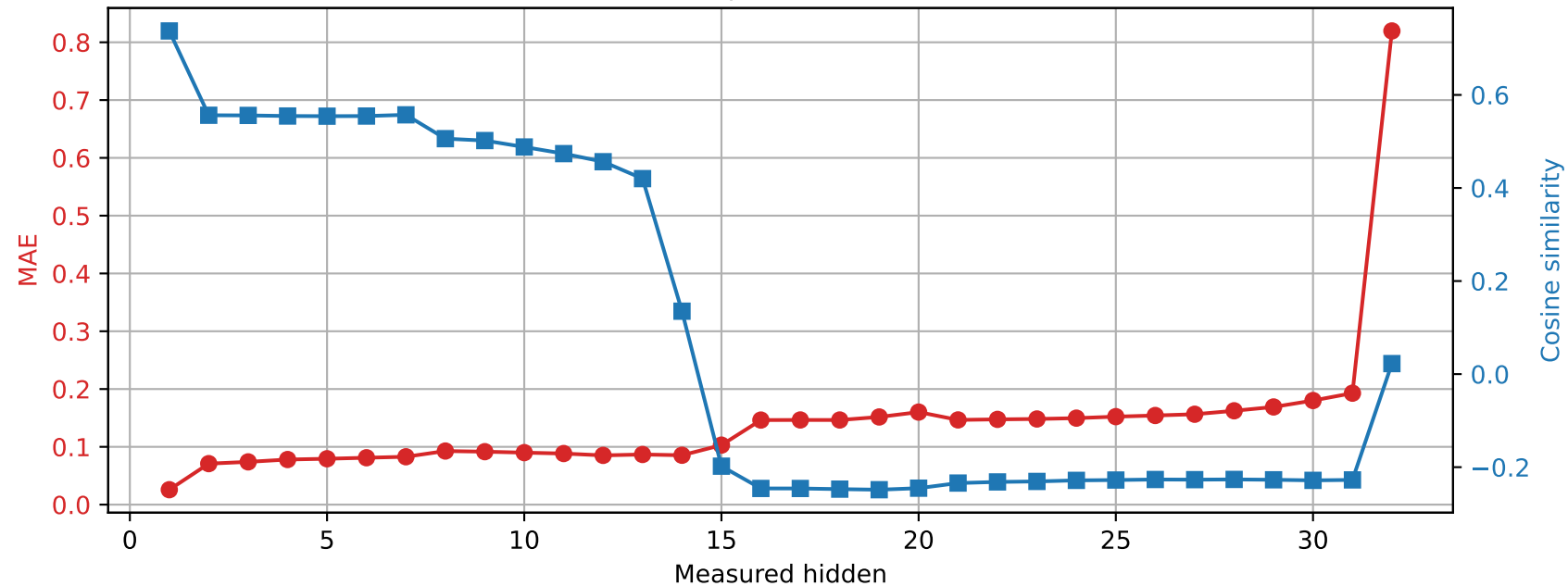
OLMo-7B-hf | Prompt 1 Spared layer 25 | Unquantized vs hybrid
