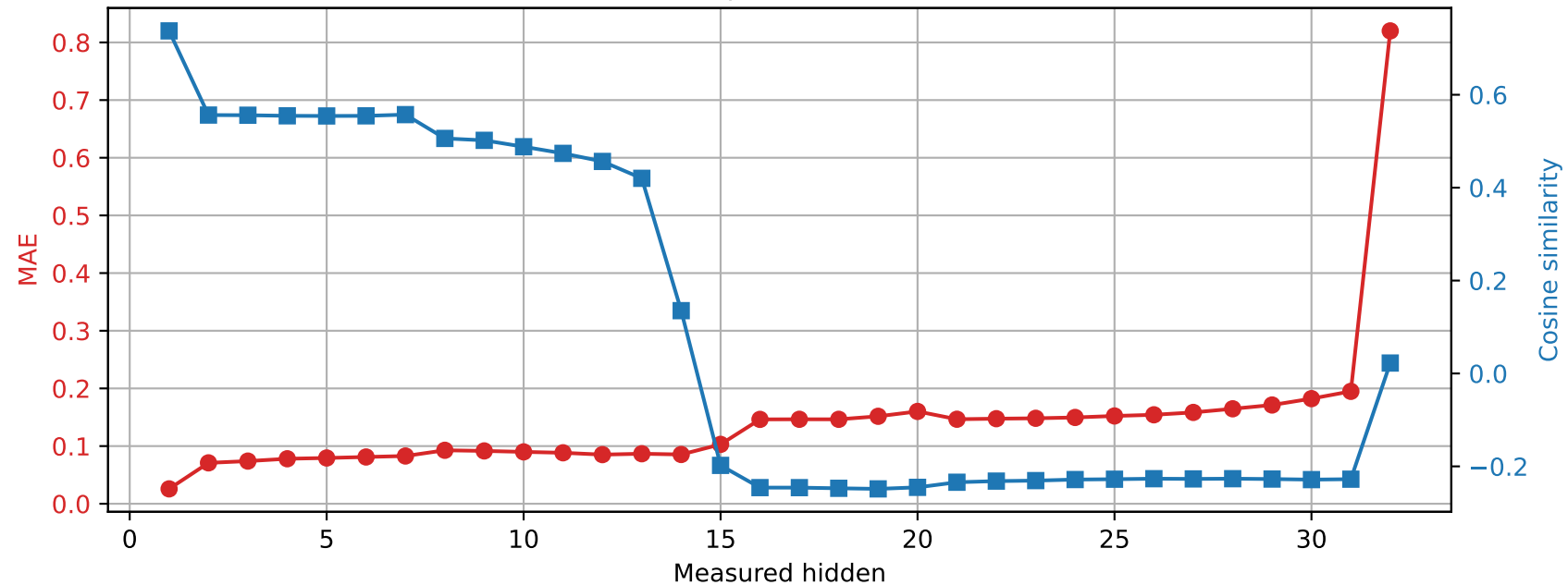
OLMo-7B-hf | Prompt 1 Spared layer 26 | Unquantized vs hybrid
