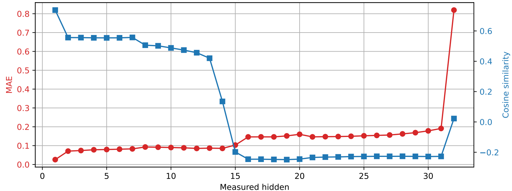
OLMo-7B-hf | Prompt 1 Spared layer 29 | Unquantized vs hybrid
