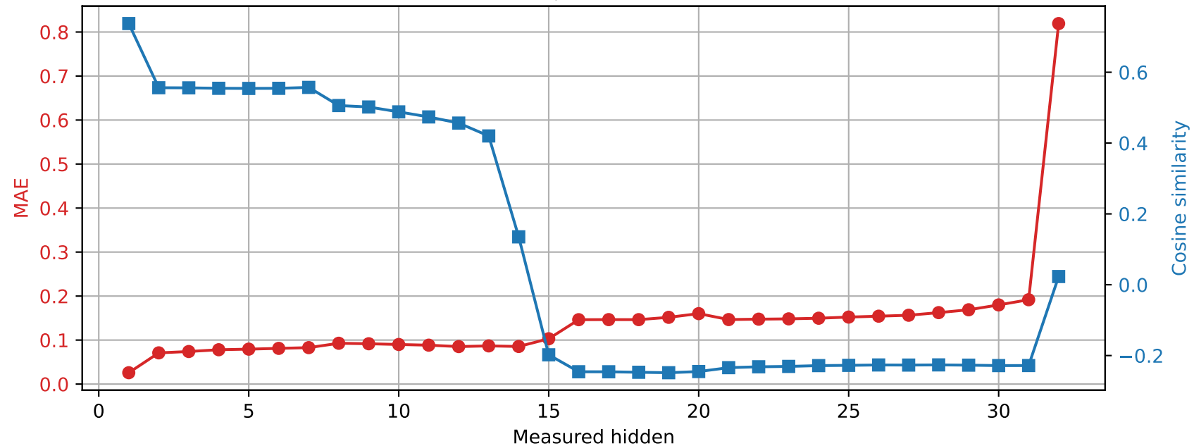
OLMo-7B-hf | Prompt 1 Spared layer 30 | Unquantized vs hybrid
