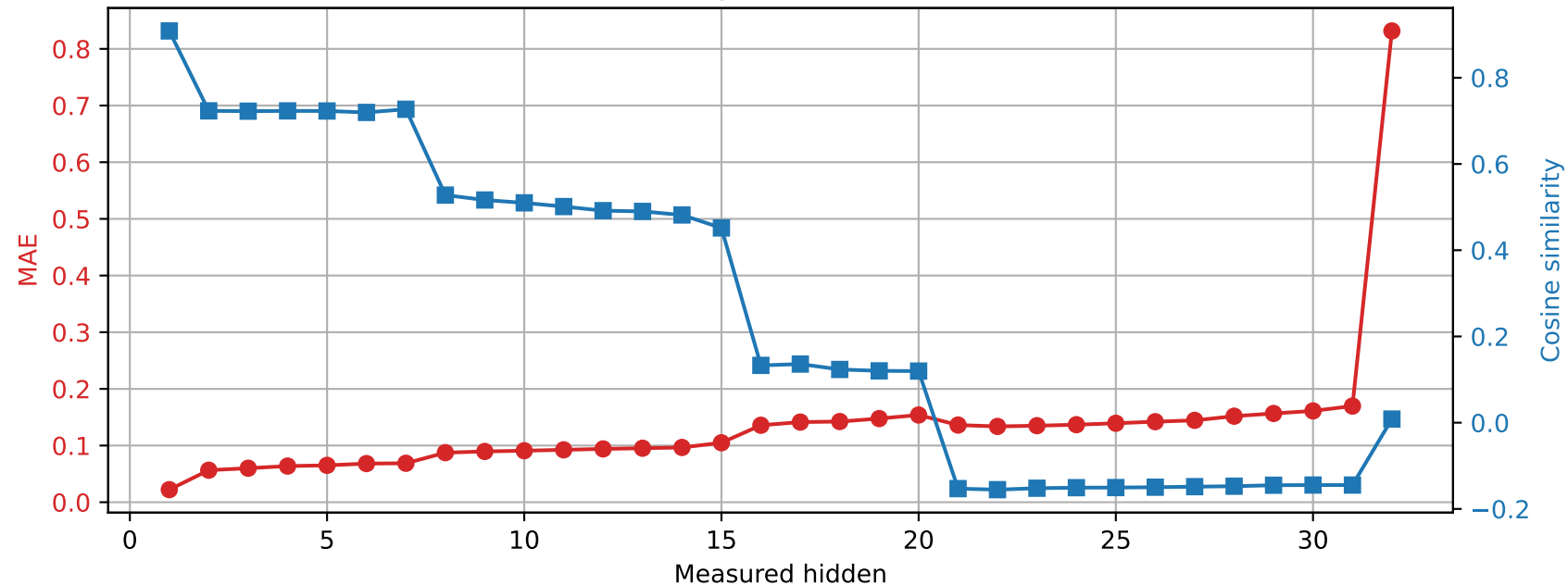
OLMo-7B-hf | Prompt 2 Spared layer 1 | Unquantized vs hybrid
