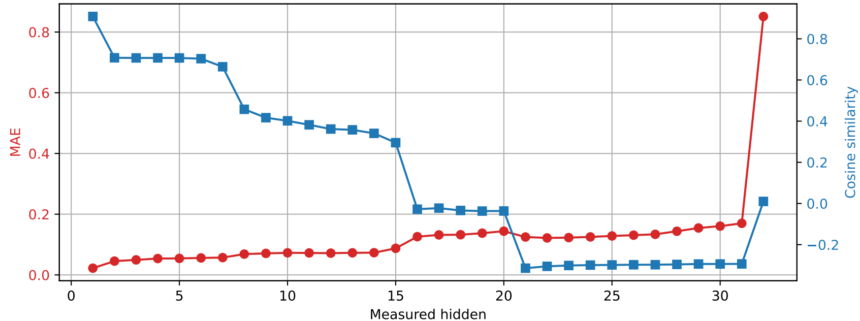
OLMo-7B-hf | Prompt 2 Spared layer 9 | Unquantized vs hybrid
