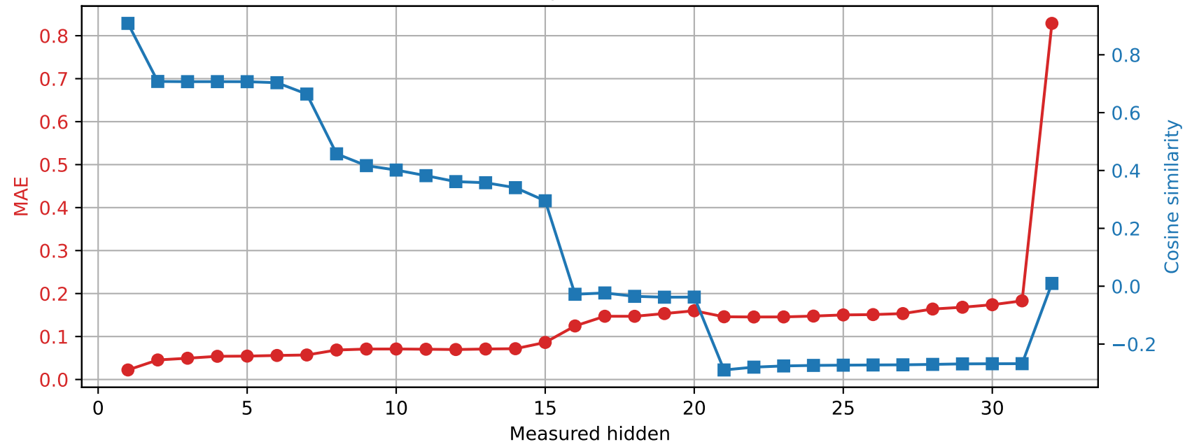
OLMo-7B-hf | Prompt 2 Spared layer 16 | Unquantized vs hybrid
