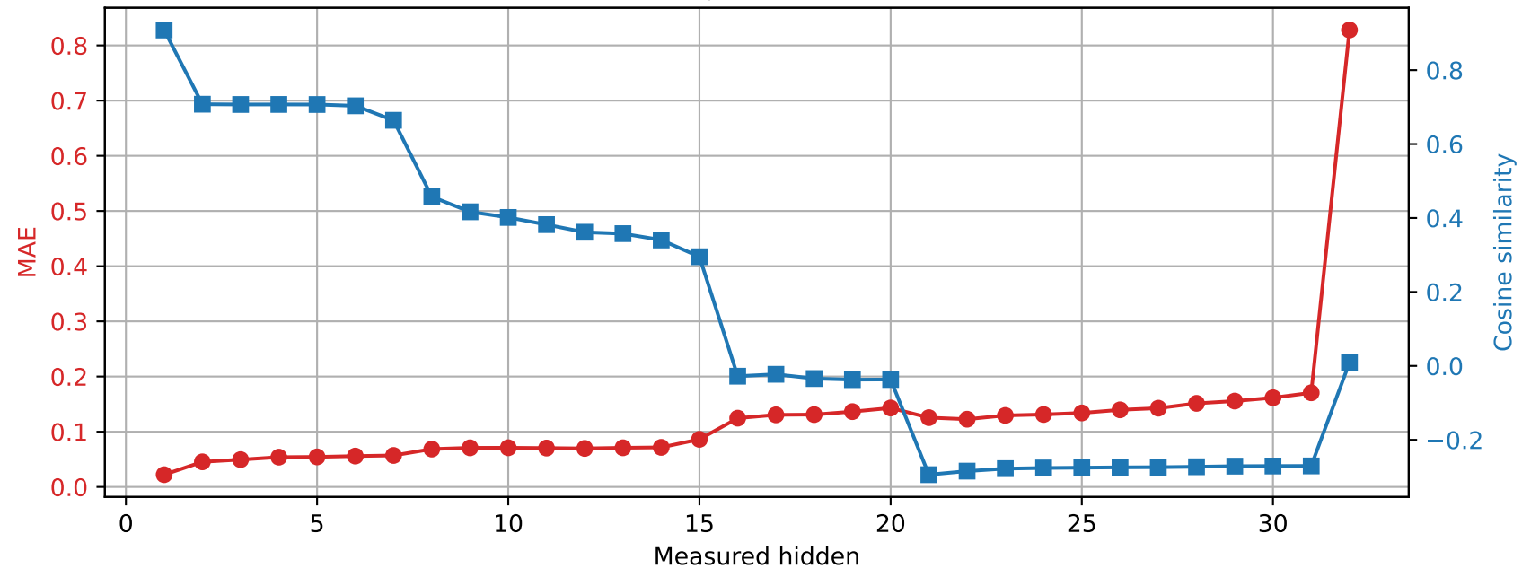
OLMo-7B-hf | Prompt 2 Spared layer 22 | Unquantized vs hybrid
