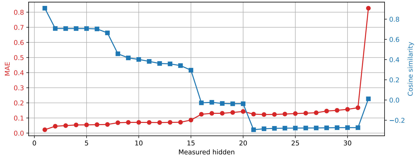
OLMo-7B-hf | Prompt 2 Spared layer 30 | Unquantized vs hybrid
